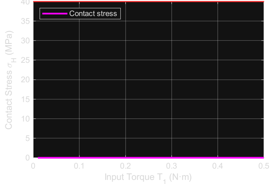
Yield = 40 MPa Hertzian Contact Stress vs Input Torque
