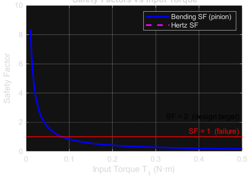
Safety Factors vs Input Torque
