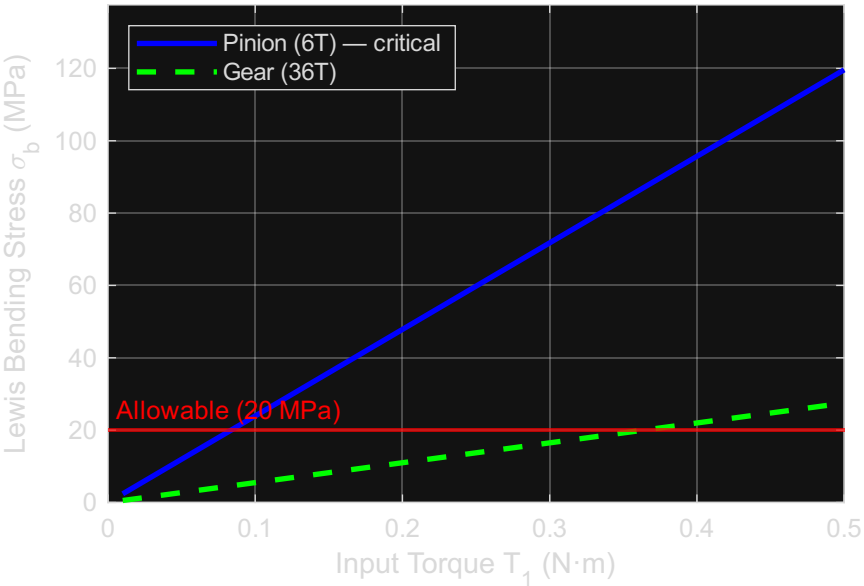
Lewis Bending Stress vs Input Torque
